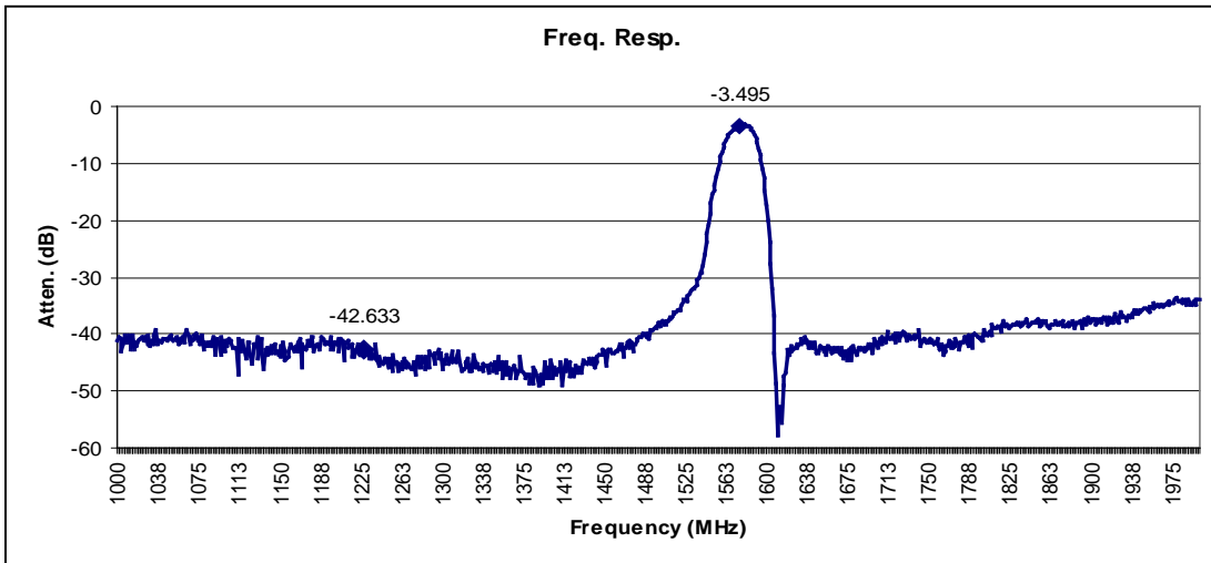
L1FT Passive Filter (High Rejection)
